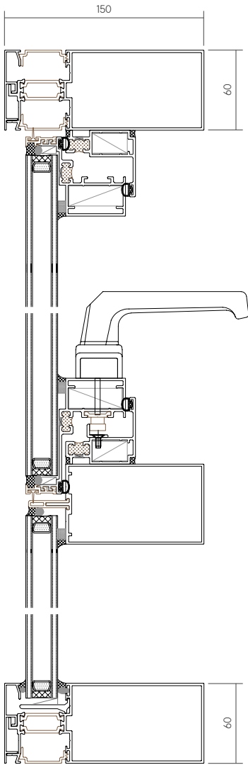
㉠ VERTICAL SECTION DETAIL
