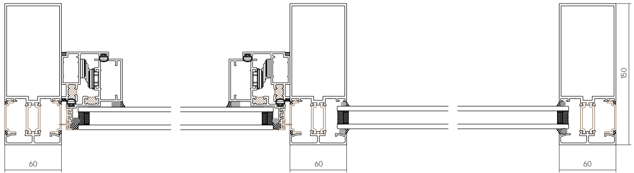
㉢ HORIZONTAL SECTION DETAIL
